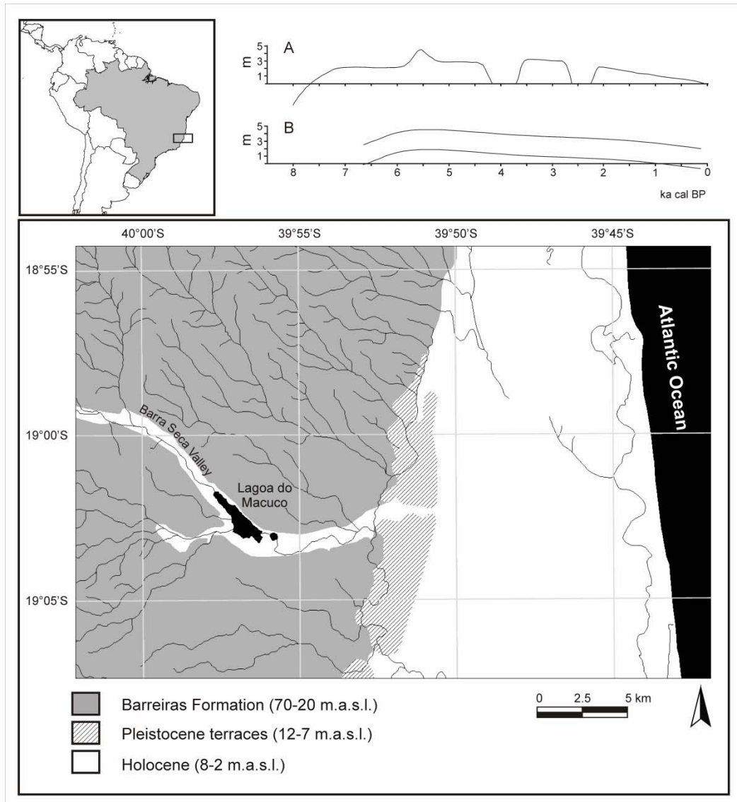
Figure 1: Study site. Map showing the location of the study site at the Brazilian coast (upper left panel), and in the geologic and elevation contexts (lower panel); relative sea-level curves for the southeastern Brazilian coast (upper right panel), in meter above present sea-level (m.a.s.l.), versus the time in thousands of calibrated years (ka cal BP); (A) subpanel from Martin et al. (2003) ; (B) subpanel from Angulo et al. (2006) .
