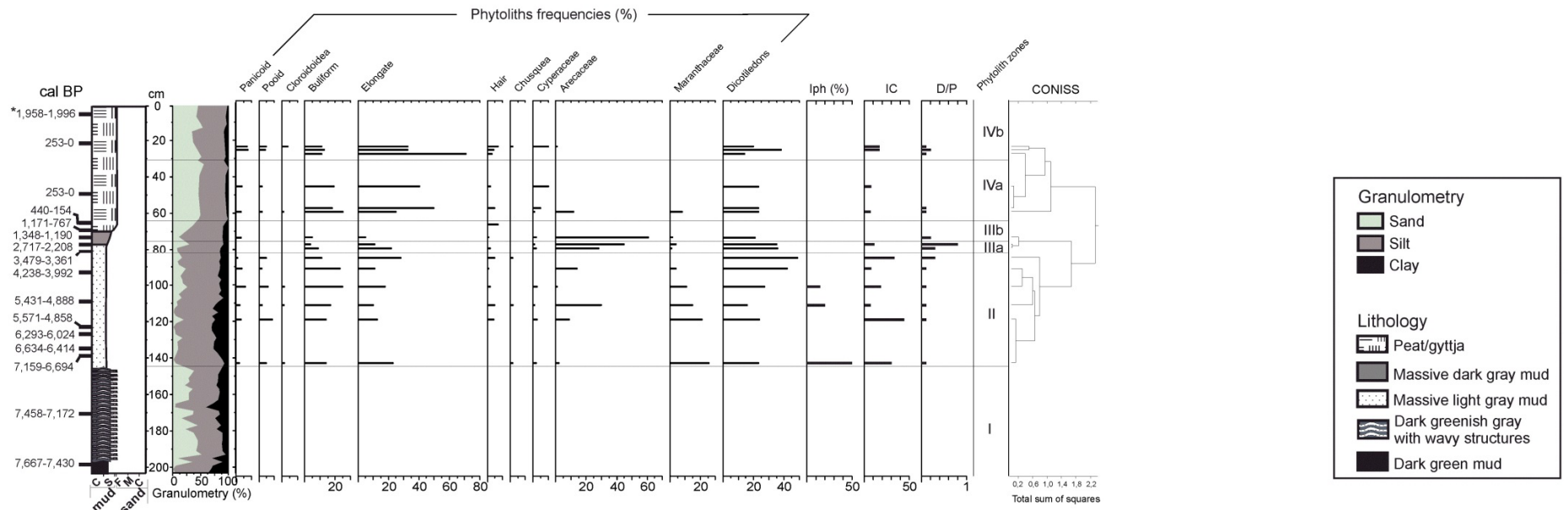
Figure 3: Calibrated ages, lithology; Phytolith percentage diagram, cluster analysis, phytolith indices and phytolith zones for the MAC-C core.
