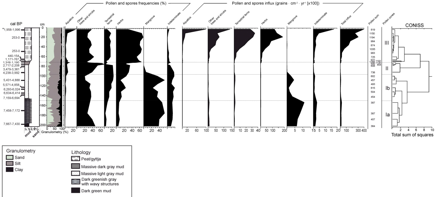
Figure 2: Calibrated ages, lithology; Pollen and spore percentage diagram, pollen and spore influx, cluster analysis, and pollen zones;
