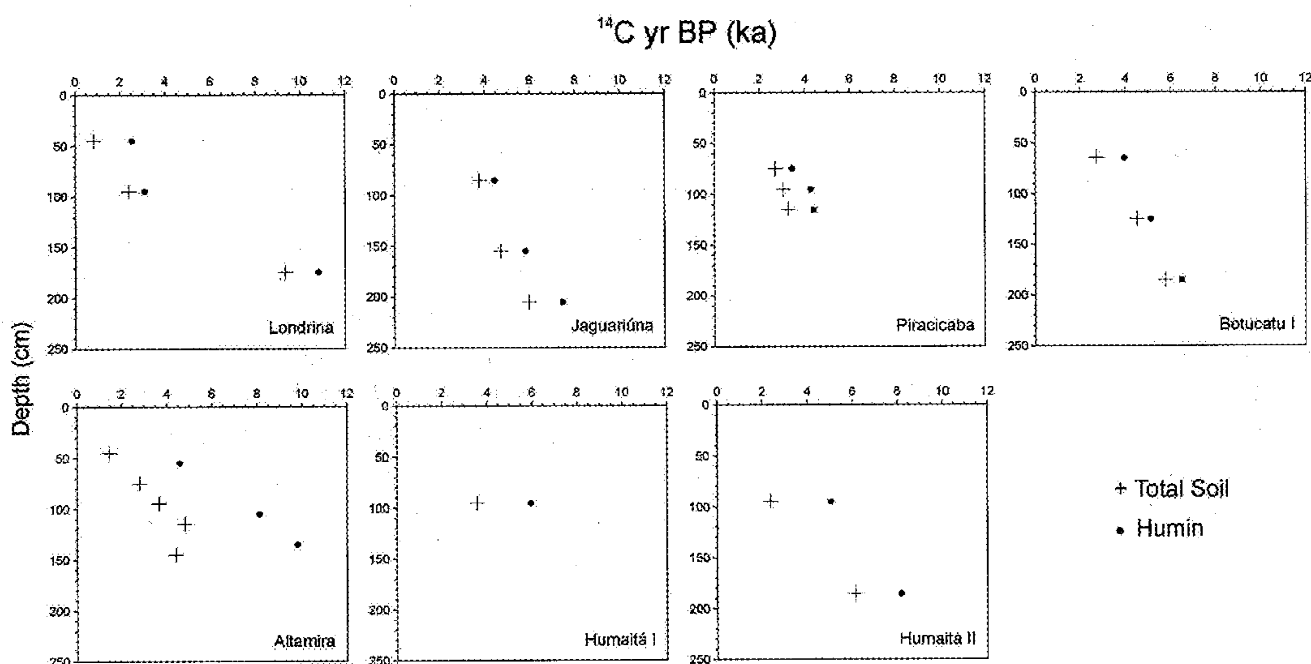
Figure 2 Comparison between total soil and humin ages
