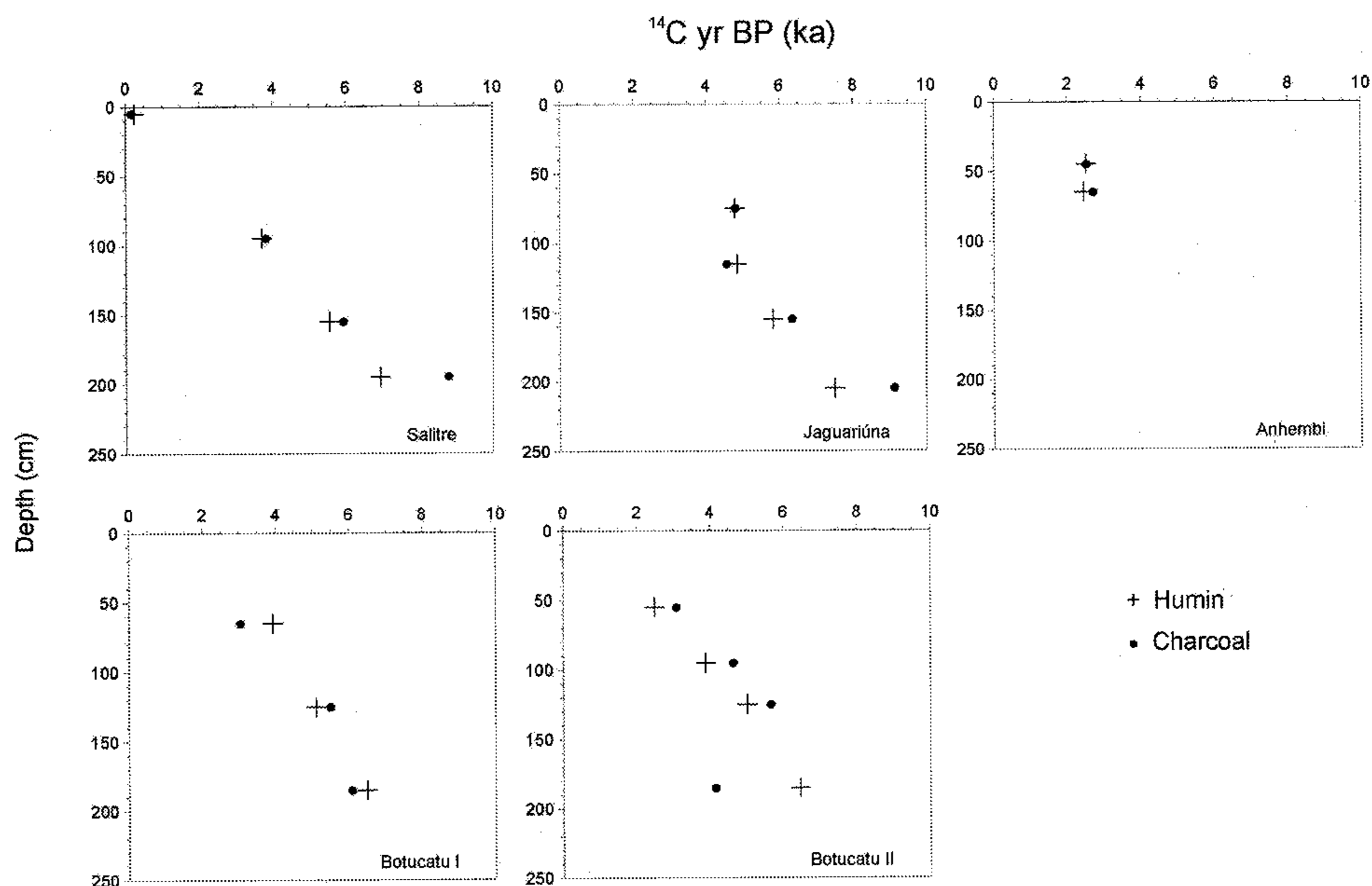
Figure 3 Comparison between the humin and charcoal ages
