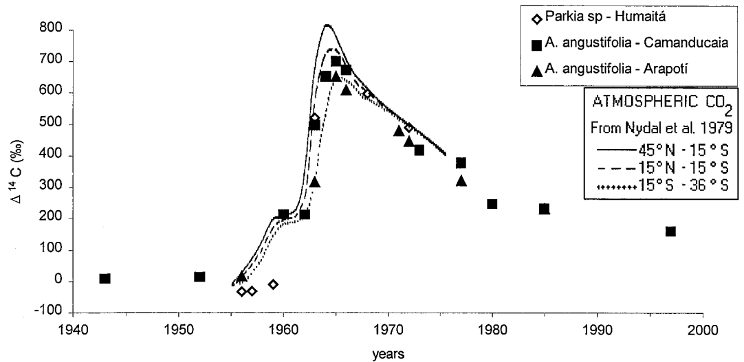
Figure 2. \Delta^{14}\text{C} in annual growth rings of Parkia sp. and A. angustifolia trees from three sites and determined by Nydal et al. (1979).
