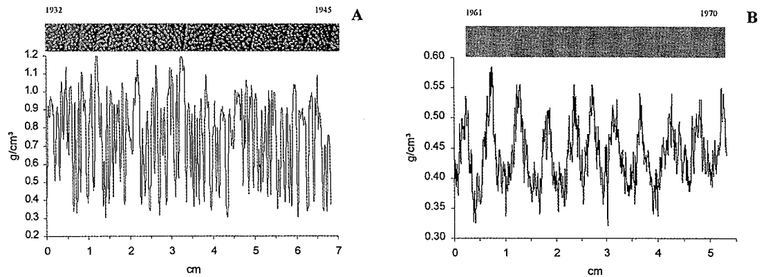
Figure 1. Wood anatomical structure and density profile by X-ray densitometry of Parkia sp. (A) and A. angustifolia (B) trees.
